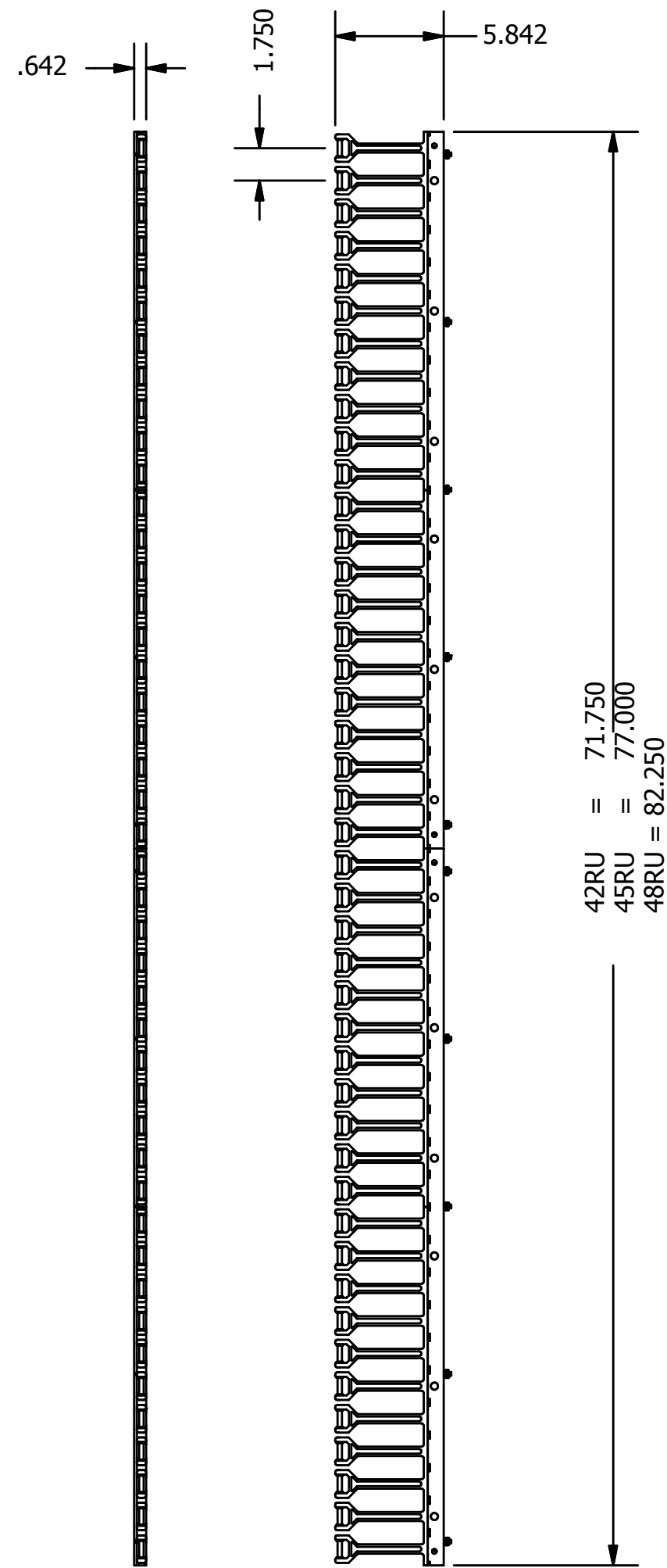
VERTICAL FINGER MANAGER STRIP (MOUNTS TO EIA RAIL)
