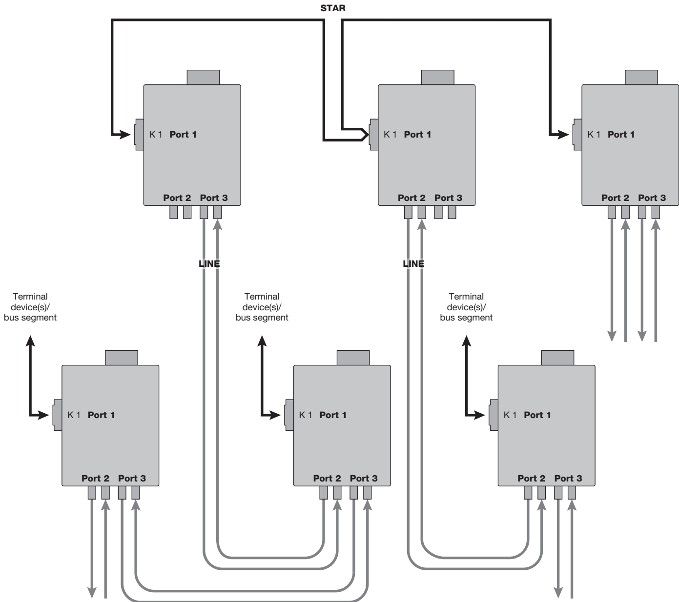
Fig. 5: Star distributor
